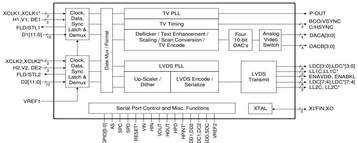
Figure 1: CH7018A Functional Block Diagram
