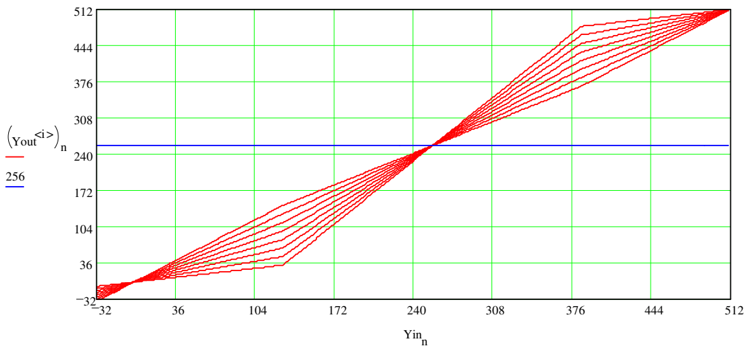
Figure 23: Contrast Enhancement of the CH7018A
