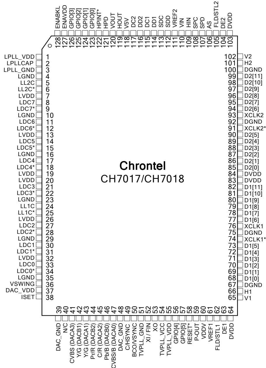
Figure 2: CH7018A 128 Pin LQFP Package (Top View)
