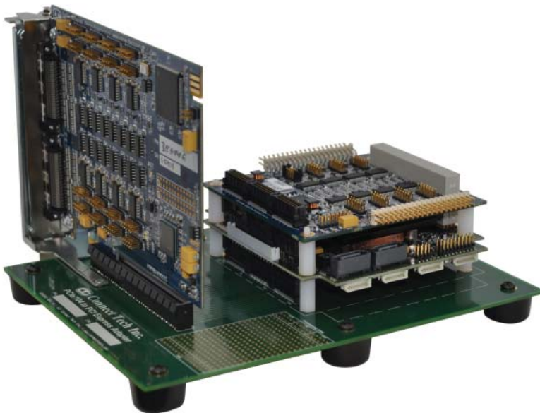
ADG021 with PCIe/104 SBC card and PCI Express card installed
