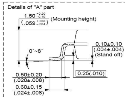
64-Lead Thin Plastic Quad Flatpack (LQFP)
