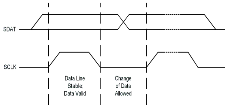
Bit Transfer on the MCU Interface
