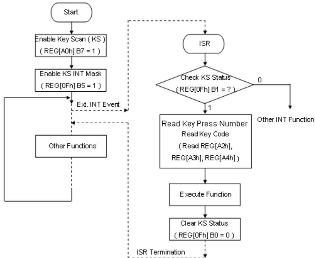
Figure 6-18 : Key-Scan Flowchart (2)
