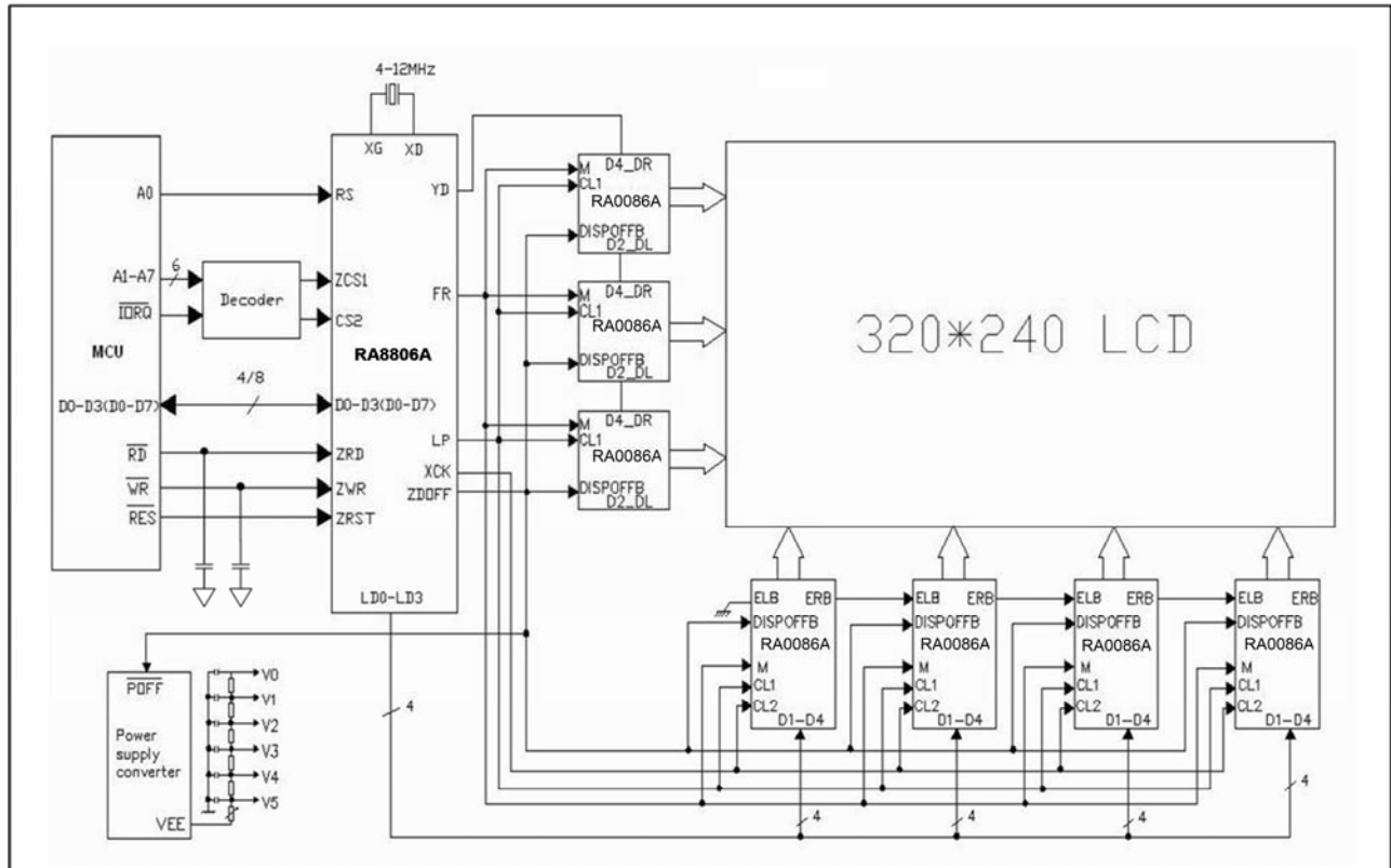
Figure 6-10 : Application Circuit Diagram for 320x240 Panel
