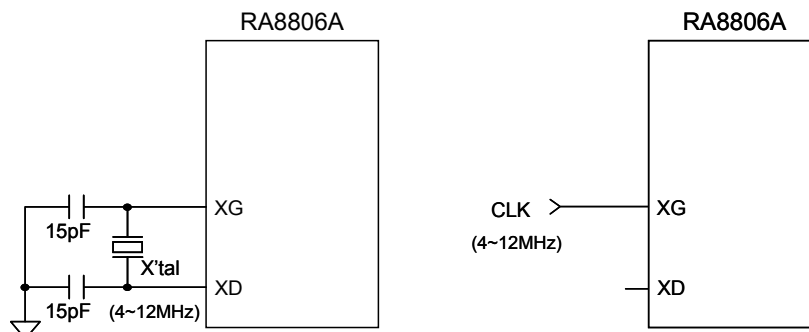
Figure 6-19 : Clock Circuit
