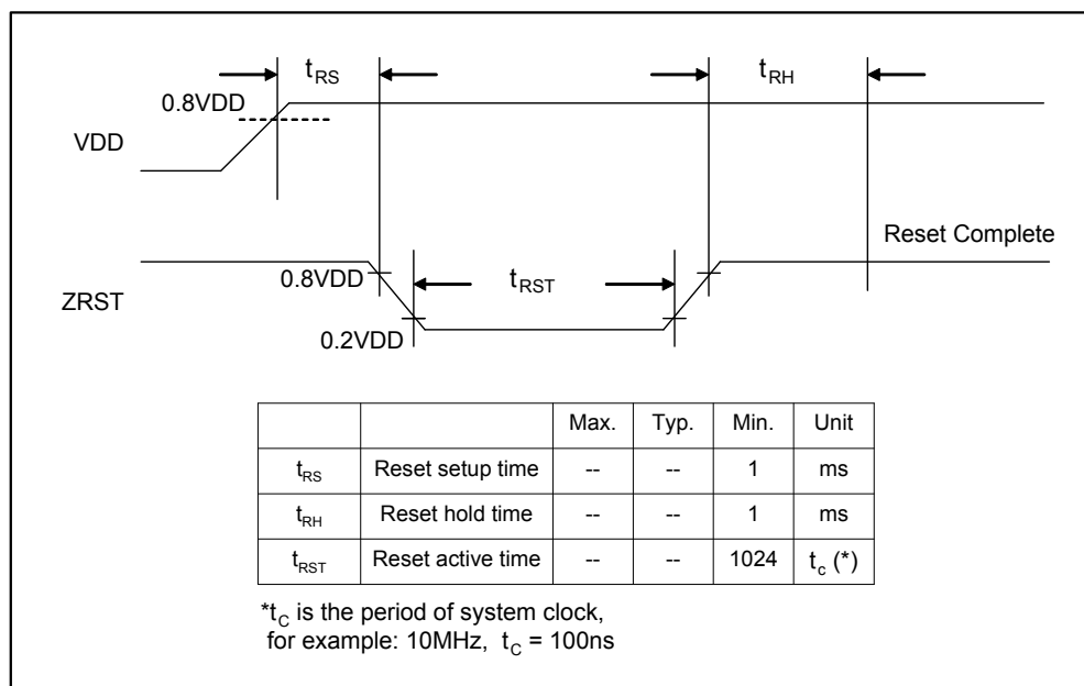
Figure 6-22 : Reset Timing
