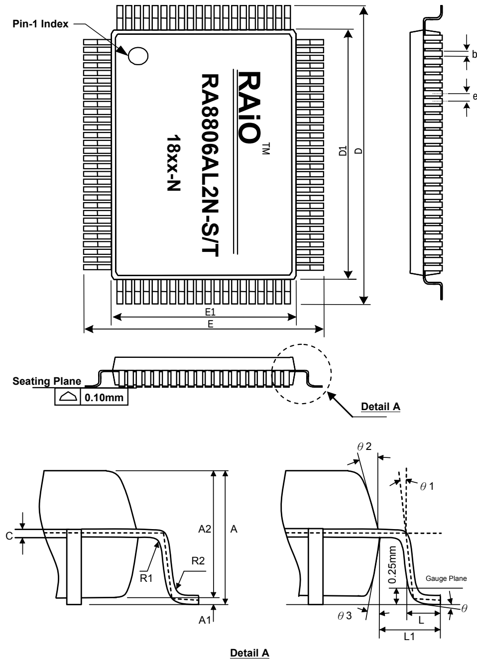
Figure 7-3 : LQFP-100Pin Mechanical
