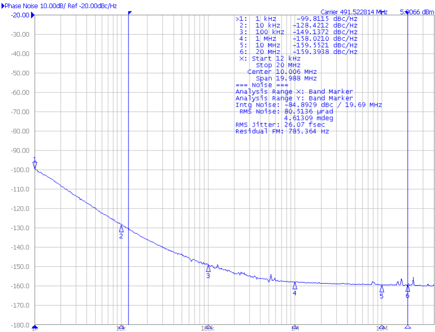
Figure 6. Center Frequency: 491.52 MHz
