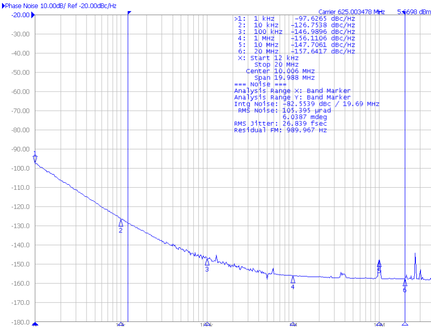
Figure 7. Center Frequency: 625 MHz
