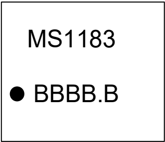
Figure 25. MS1183 Device Top Marking Showing Pin 1
