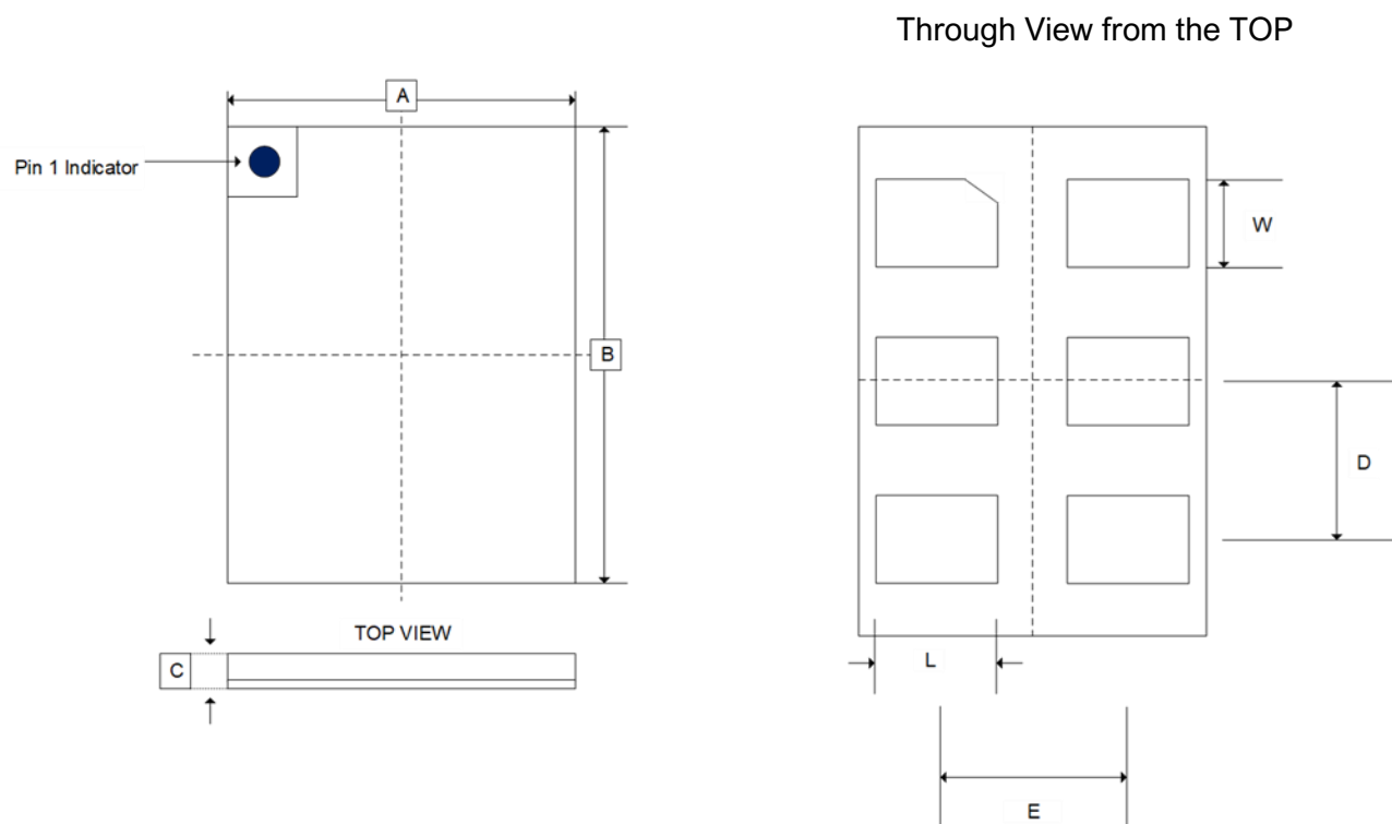
Figure 20. MS1135 Packaging Drawing (2.5X2.0 mm)
