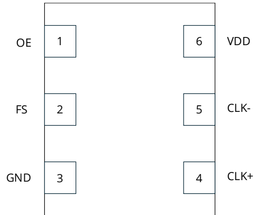
Figure 2. MS1135 Pin Assignments
