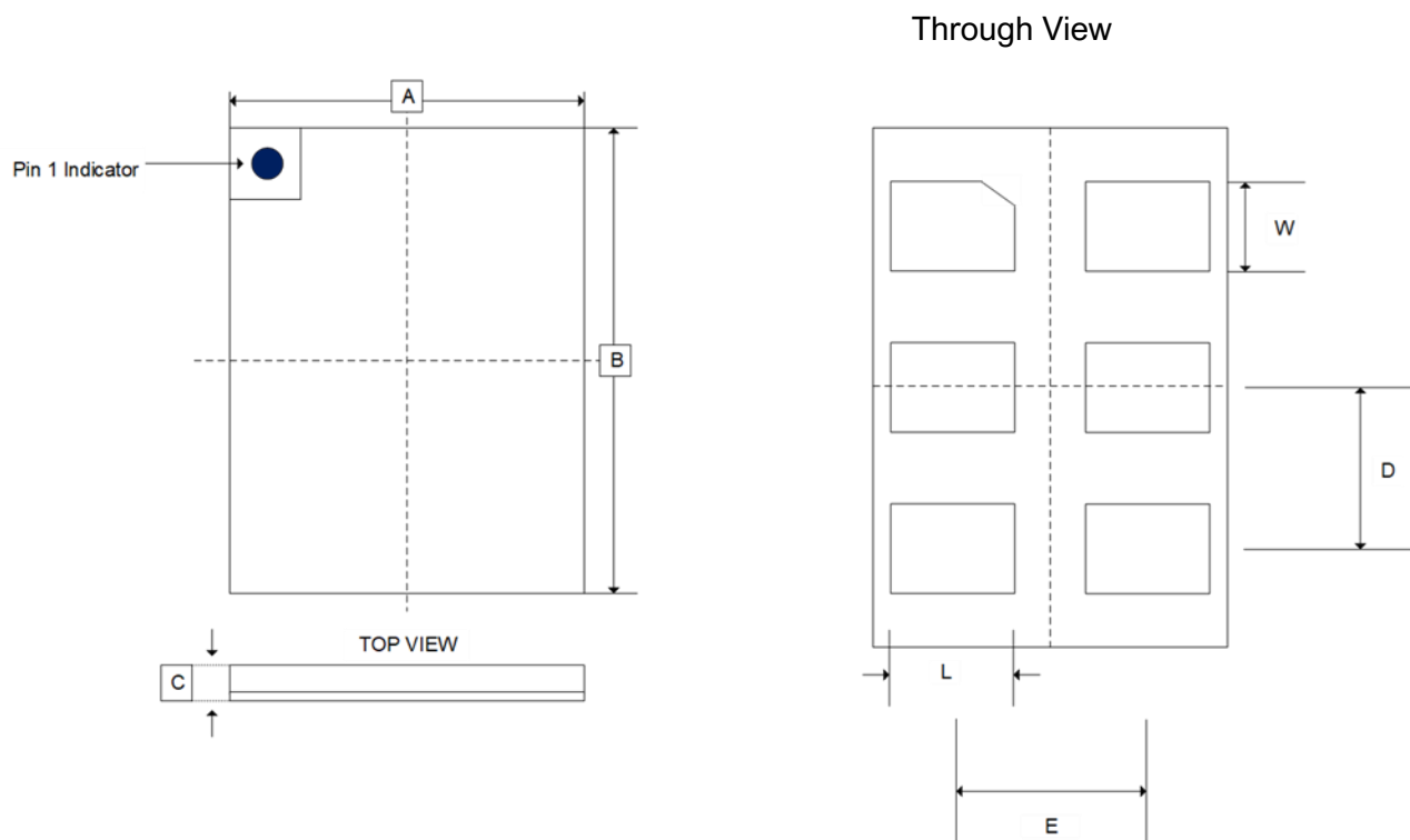
Figure 22. MS1190 Packaging Drawing (2.0X1.6 mm)
