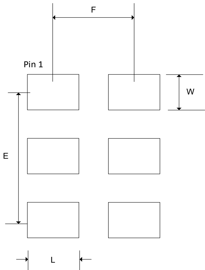
Figure 23. MS1190 Packaging Land Pattern Drawing (2.0X1.6 mm)
