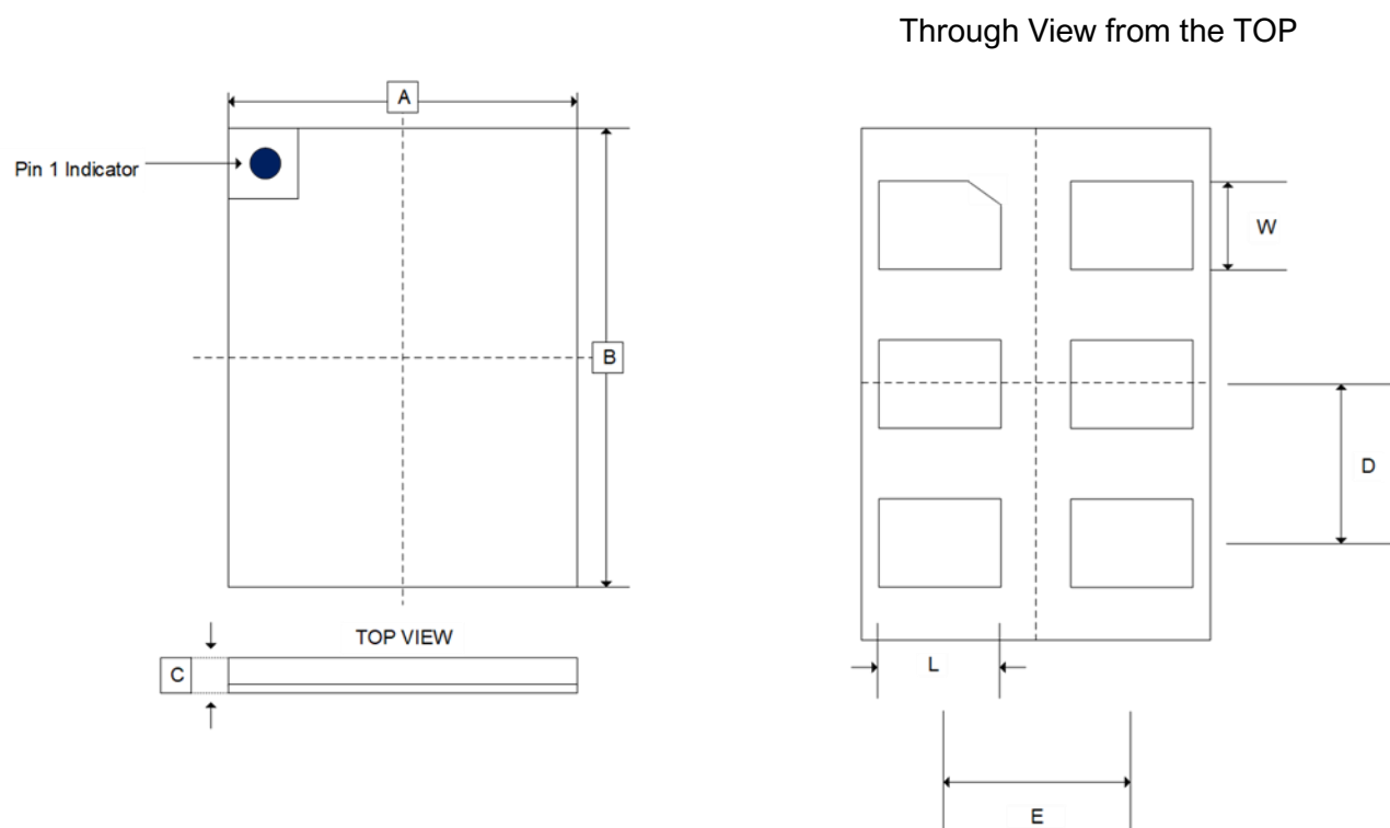
Figure 20. MS1150 Packaging Drawing (2.5X2.0 mm)
