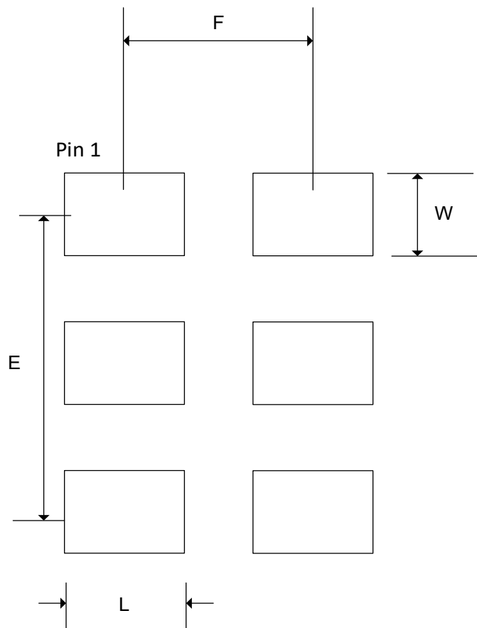
Figure 21. MS1150 Packaging Land Pattern Drawing (2.5X2.0 mm)
