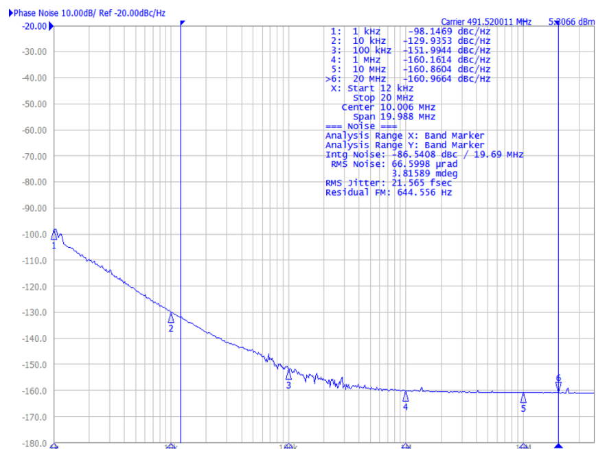
Figure 5. Center Frequency: 491.52 MHz
